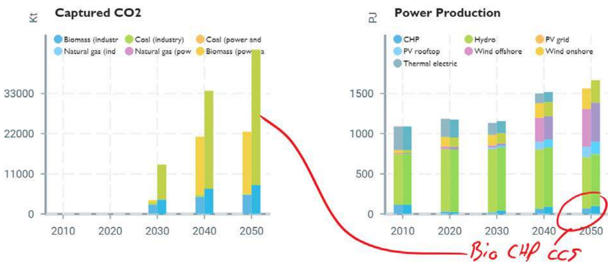
Figure 58: CCS and power production.
